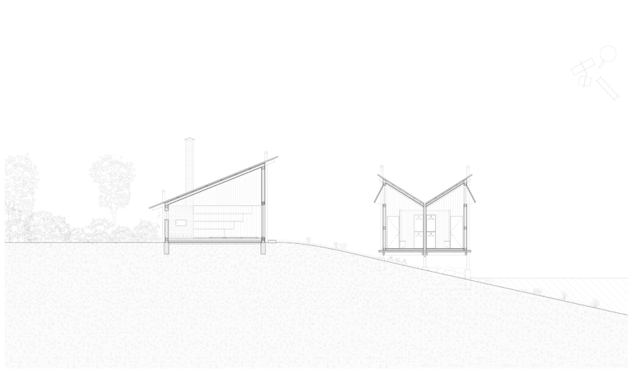
Section AA 1:50
