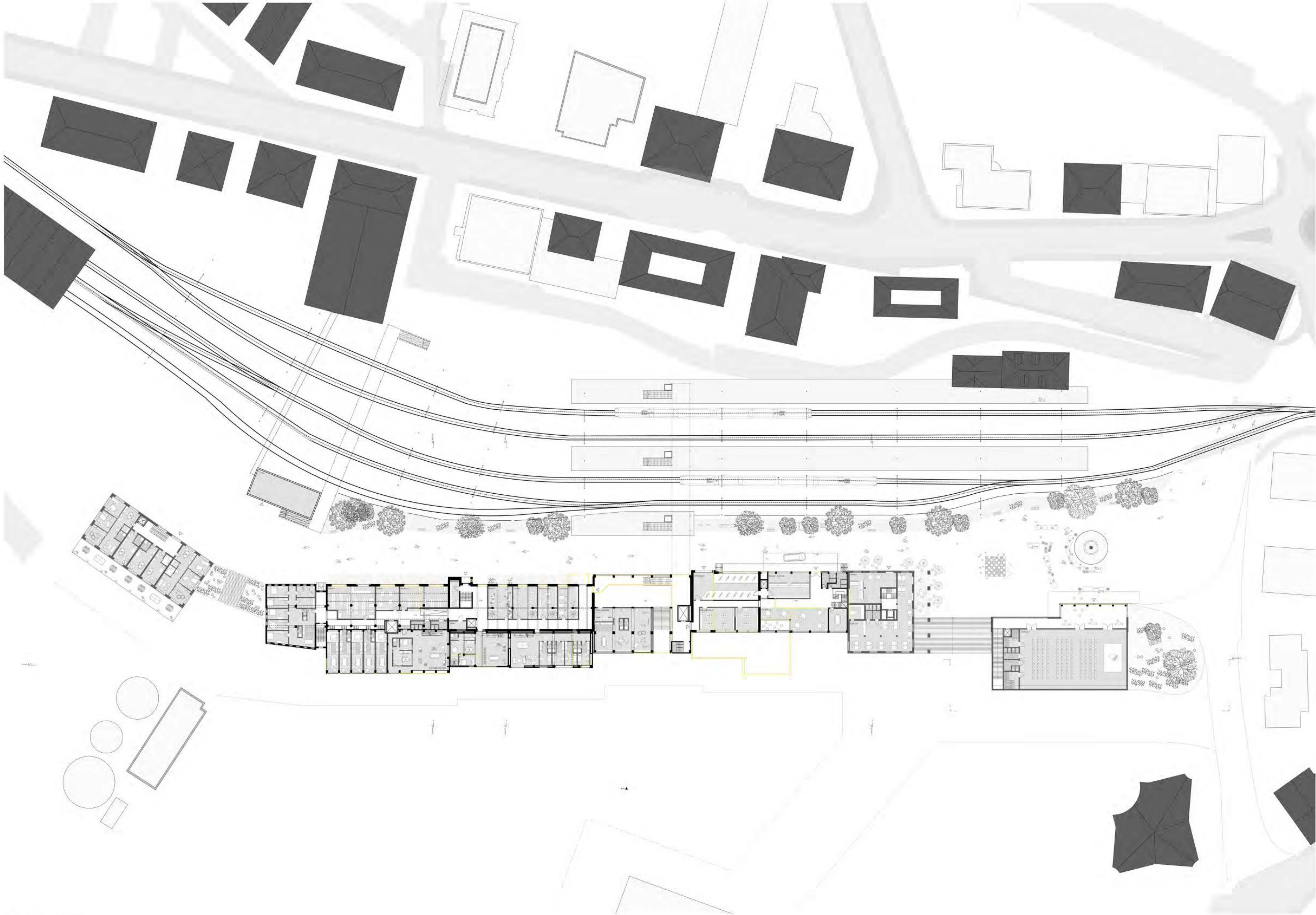
Situation| Mst. 1:400
