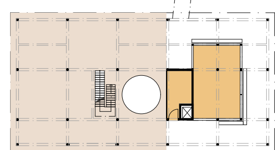
Schemaplan - Erdgeschoss | 1:500
