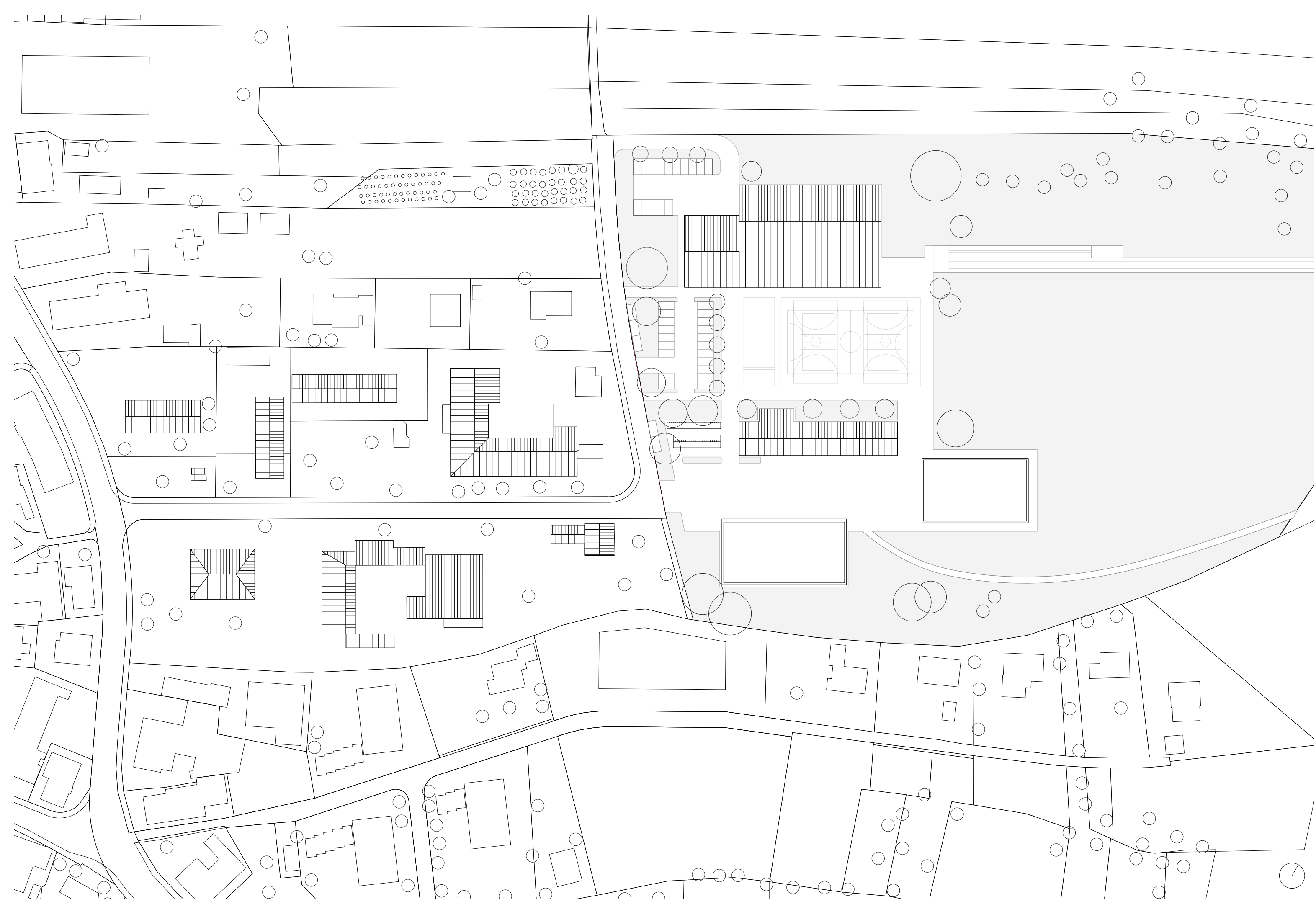
Situationsplan
